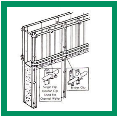
Wall Formwork System
