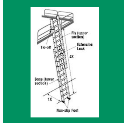
Extension Ladders
